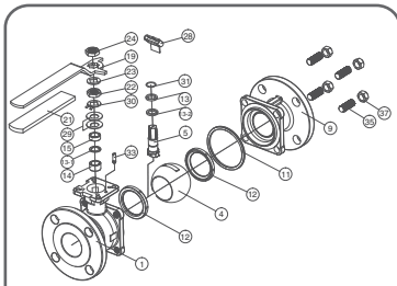
Explosion Drawing
