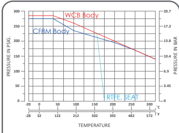
Class 150# P-T Chart
